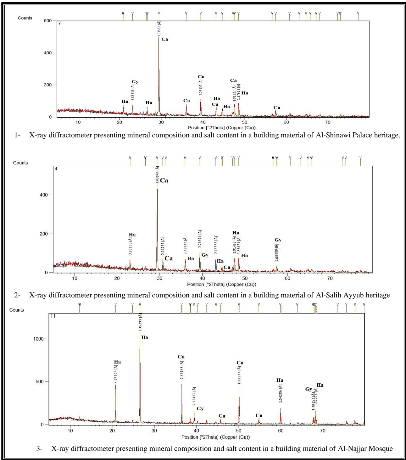
Figure 16. X-ray Analysis of Stone Samples of Heritage buildings in Mansoura city
